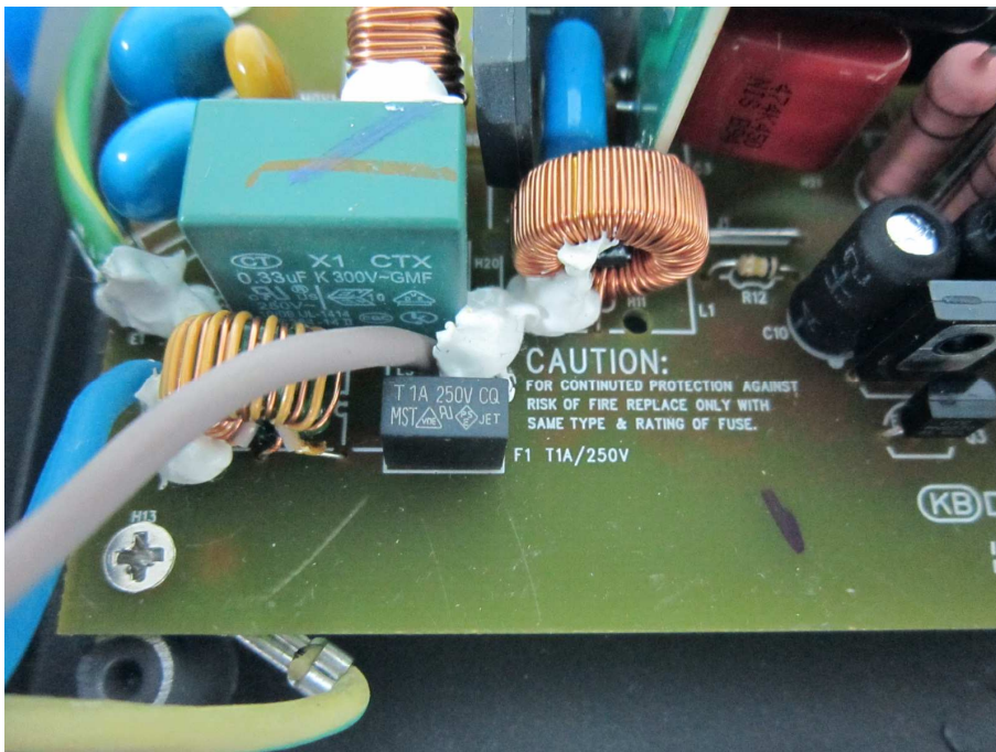
IPx4 after the test
